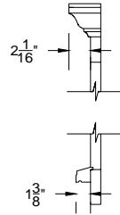
Cross Section, Head & Sill
