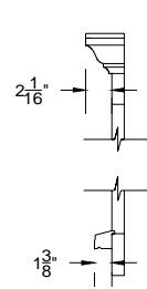
Cross Section, Head & Sill
