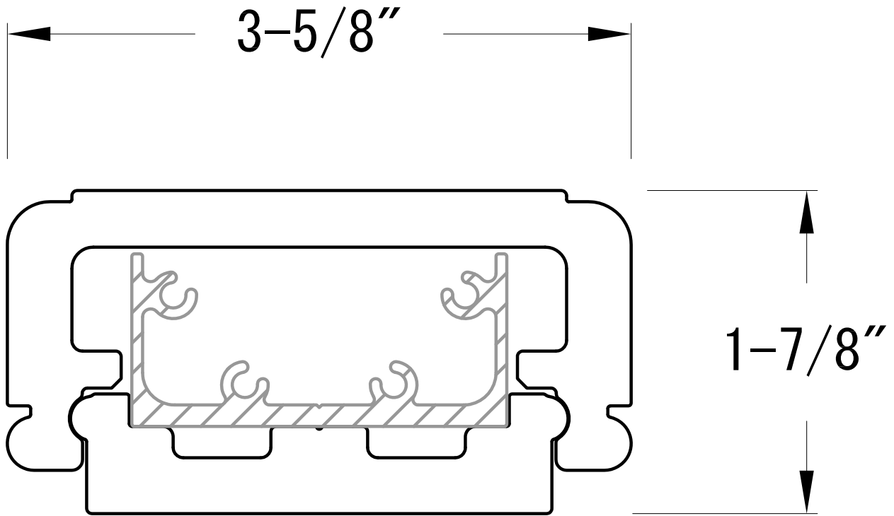
Top Rail RS35350
