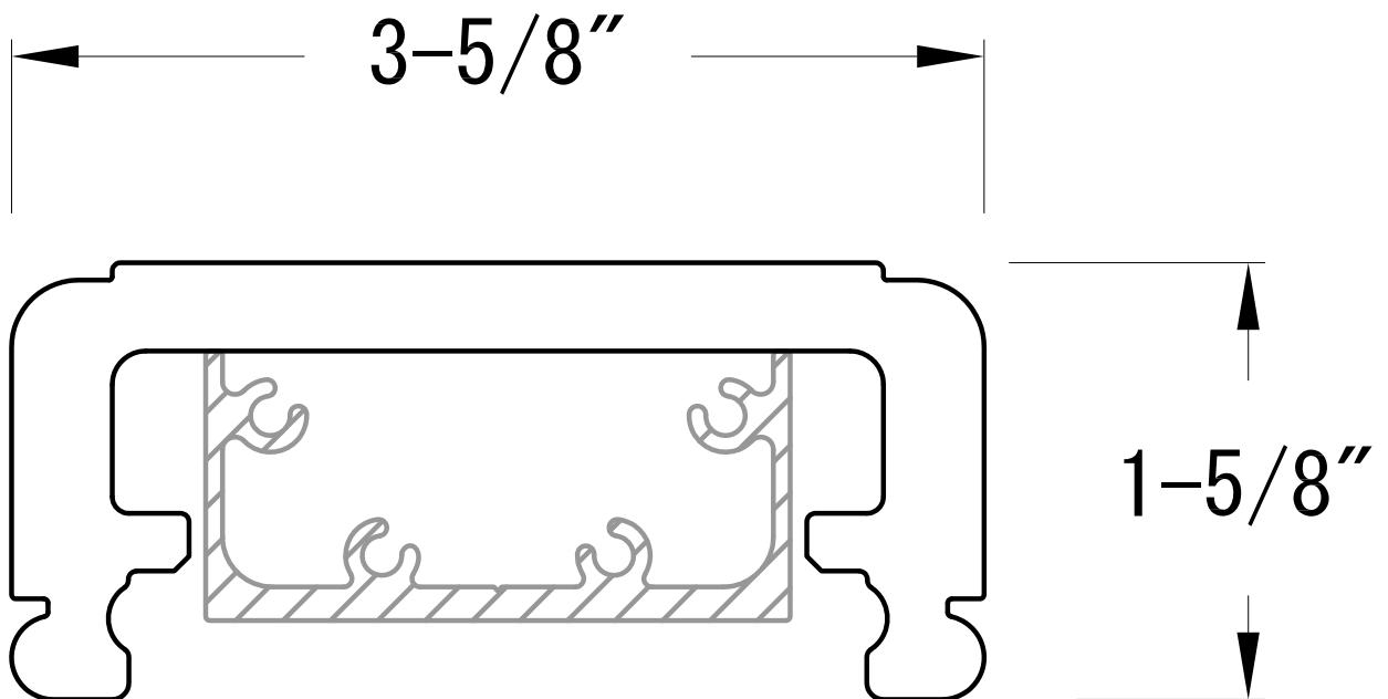
Bottom Rail RS35400
