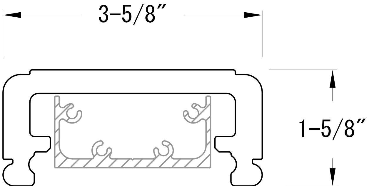
Bottom Rail RS35350
