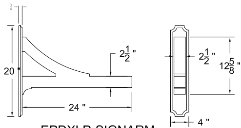
EPDXLP-SIGNARM Optional Sign Arm
