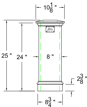
EPDXLP-FPB Flush Panel - Adder Deluxe Lamp Post
