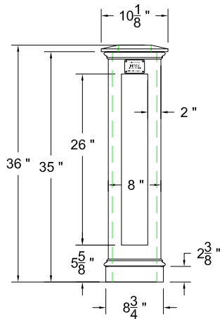
EPDXLP-RPB Recess Panel - Adder Deluxe Lamp Post
