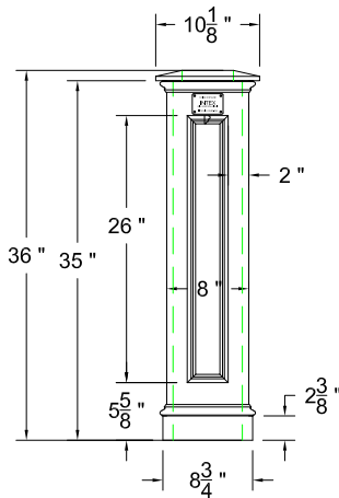
EPDXLP-RPBP Recess Panel with Plants - Adder Deluxe Lamp Post
