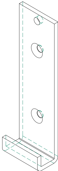
ITEM B HANGER BRACKET
